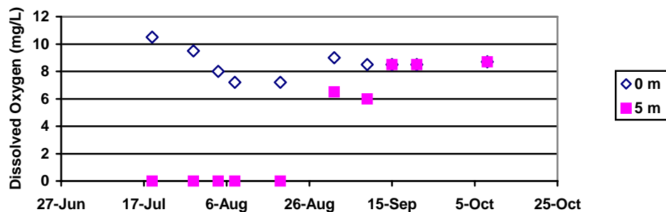
Figure 8: Temporal distribution of surface and near-bottom concentrations of dissolved oxygen in Lake Como (Effler et al., 1988).
