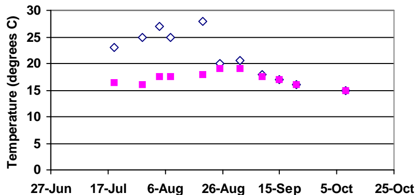
Figure 7: Temporal distributions of Surface and Near Bottom Temperatures of Lake Como (Effler et al, 1988).
