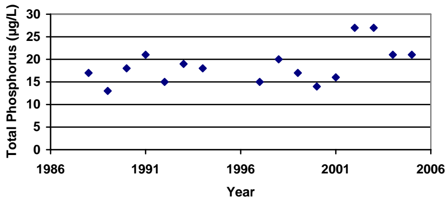
Figure 9: Average Total Phosphorus in µg/L by Year (NYFOLA and NYSDEC, 2006)
