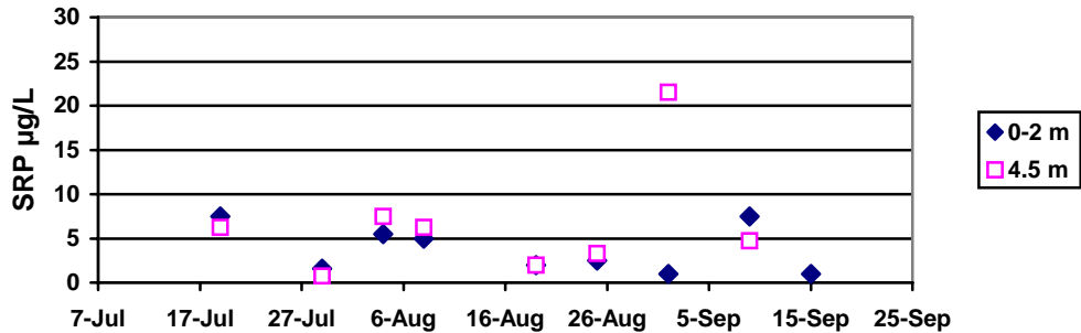
Figure 11: Soluble Reactive Phosphorus (SRP) in \mu\text{g/L} by Depth from Effler et al., 1988.
