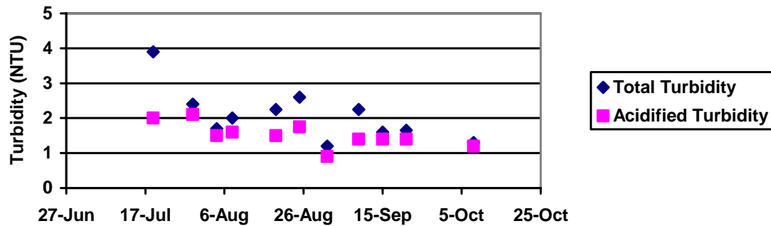
Figure 20: Temporal distributions of turbidity and acidified turbidity in the 0 to 2 meter interval of Lake Como in 1987 (Effler et al, 1988).
