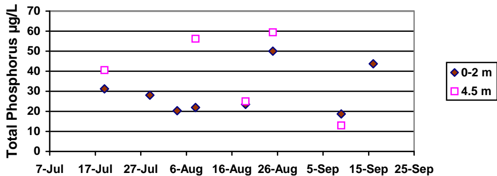
Figure 10: Total Phosphorus in µg/L by Depth from in 1987 (Effler et al., 1988)
