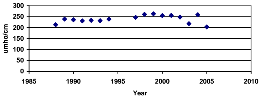
Figure 16: Average Specific Conductance Corrected to 25°C in \mu\text{mho/cm} (NYSFOLA and NYSDEC, 2006)
