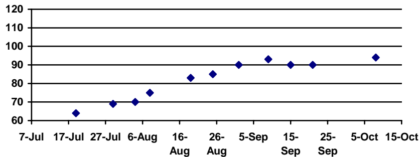
Figure 18: Alkalinity over the Course of a Summer (Effler et al., 1988)
